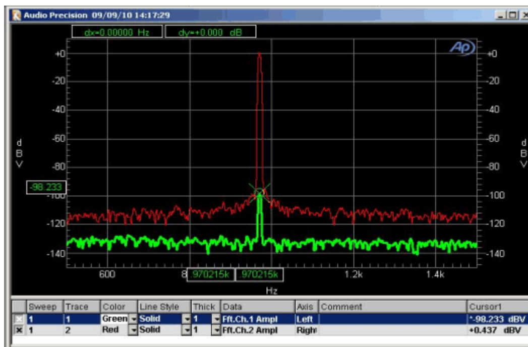
Figure 7. Crosstalk FFT
